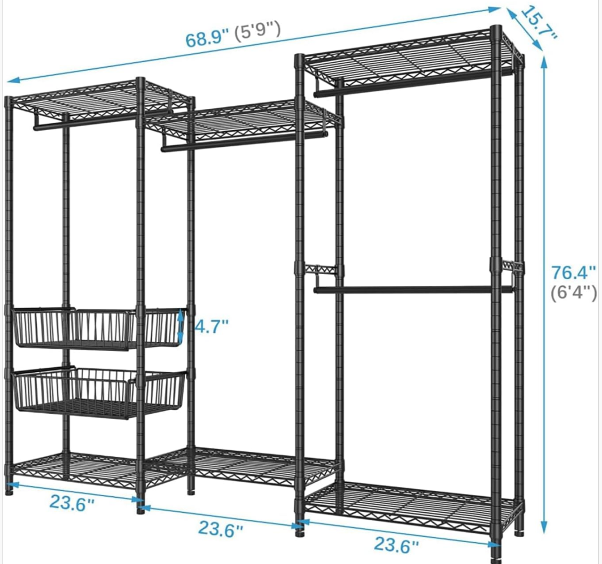
Image 2: Product dimensions diagram, illustrating the overall measurements of the VIPEK V10 Garment Rack.
