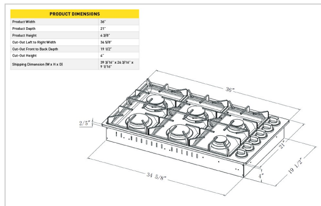
Figure 4.1: Technical drawing detailing the product width, depth, height, and the required countertop cut-out dimensions for installation.
