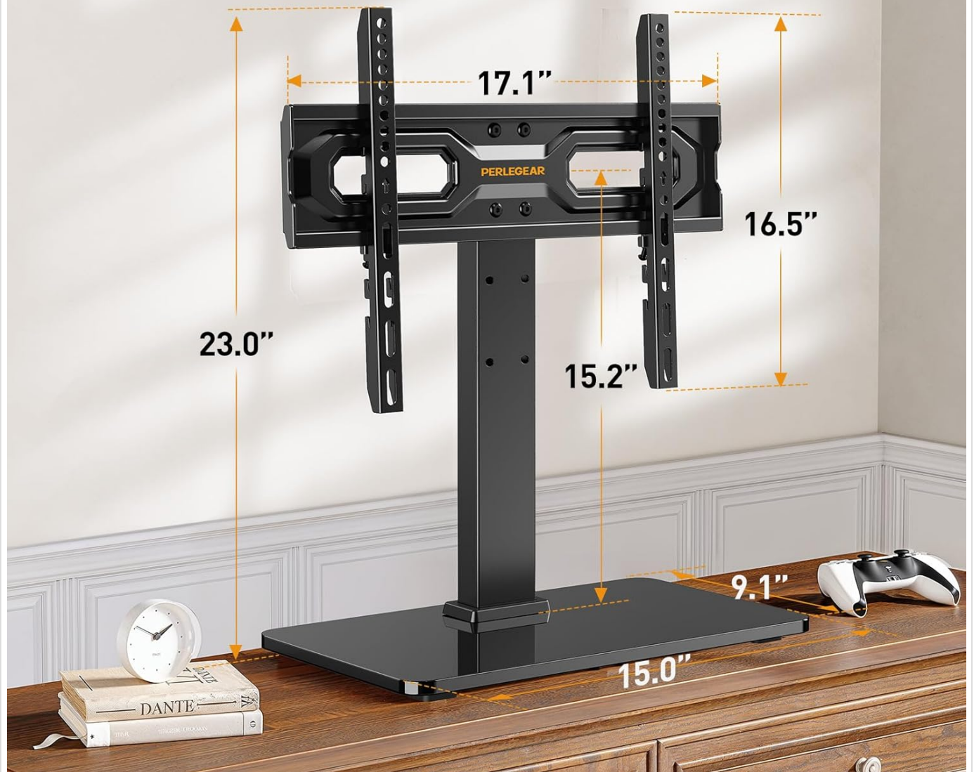
Image: Detailed dimensions of the Perlegear PGTVS02 TV stand, including height, width, and base measurements.
