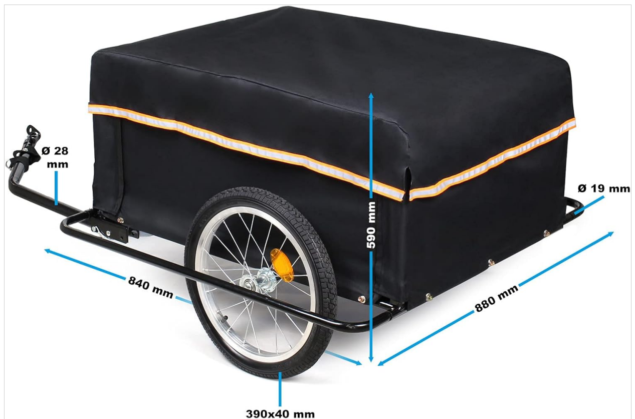
Image: The trailer with its protective cover, illustrating its overall dimensions.
