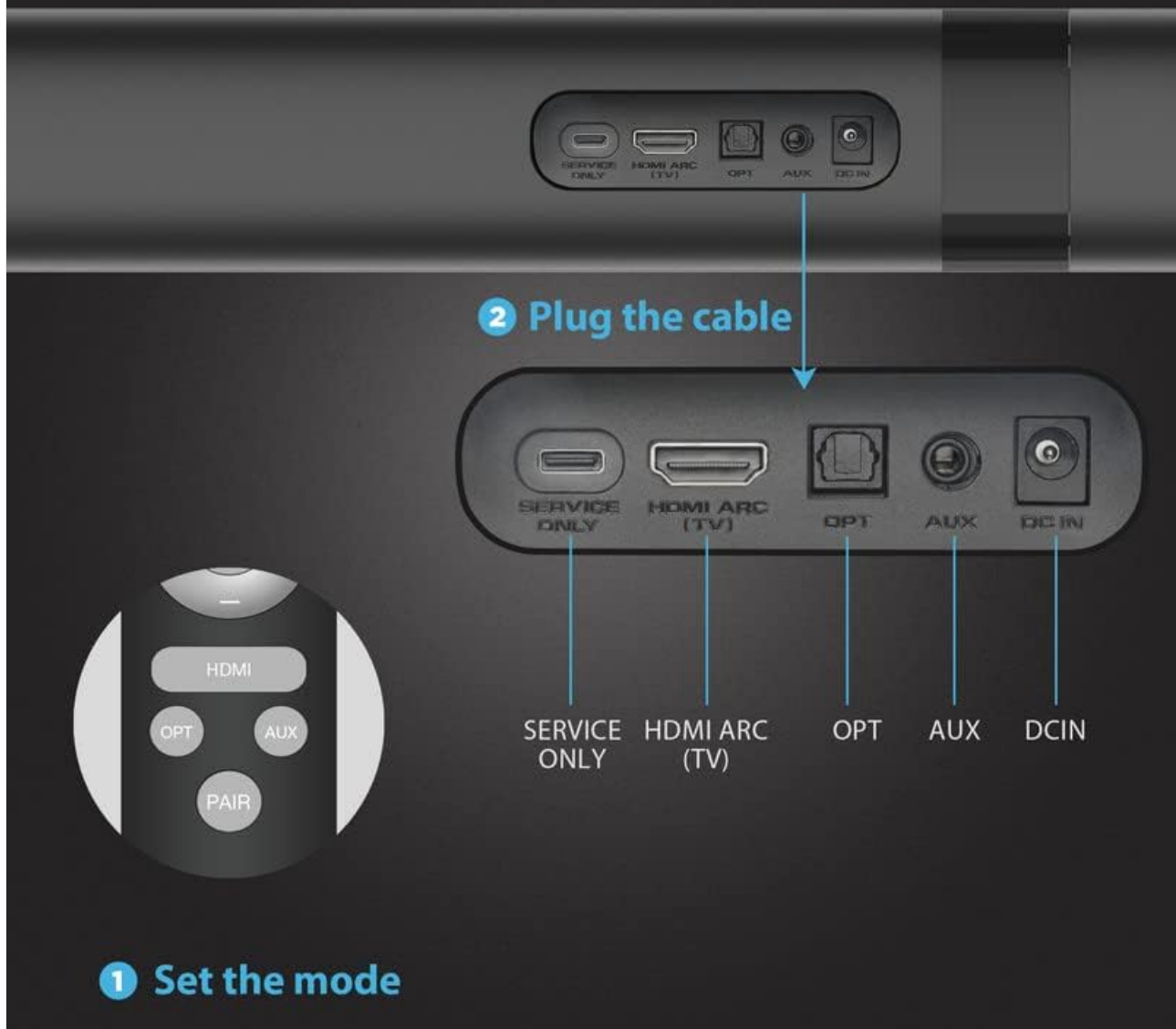
Figure 6: Detailed view of the sound bar's rear ports (Service Only, HDMI ARC (TV), OPT, AUX, DC IN) and the remote control, highlighting the simple two-step process: 1) Set the mode on the remote, 2) Plug in the cable.
