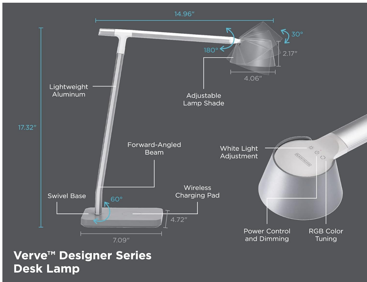
Figure 3: Lamp dimensions and adjustable components.
