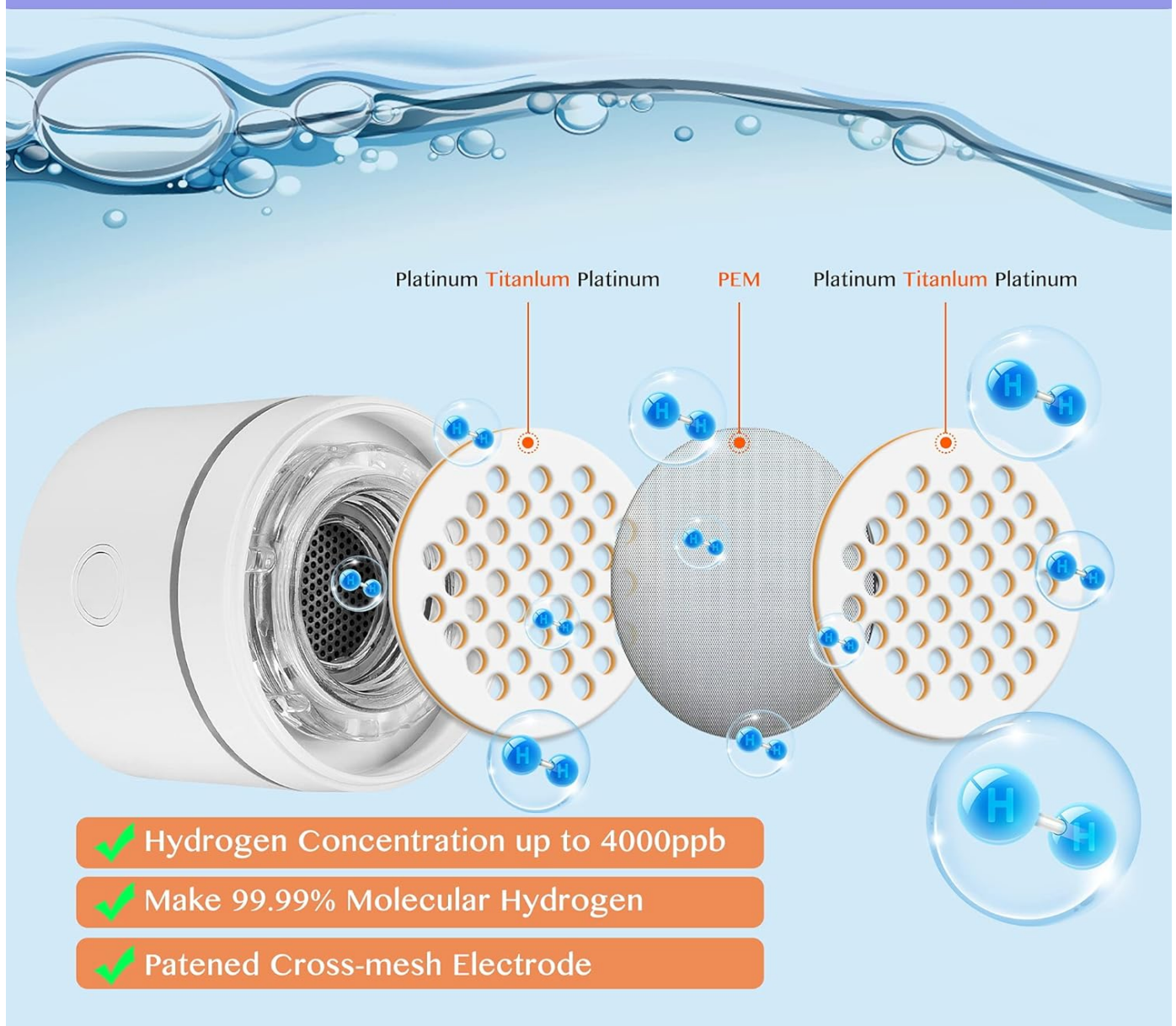
Figure 4: Illustration of hydrogen ( H_2 ) molecules being infused into the water during the generation process.
