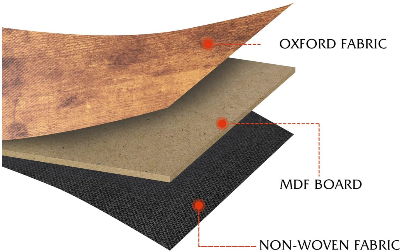
Image 6.1: Cross-section view of the drawer material, highlighting the durable Oxford fabric and non-woven fabric layers.
