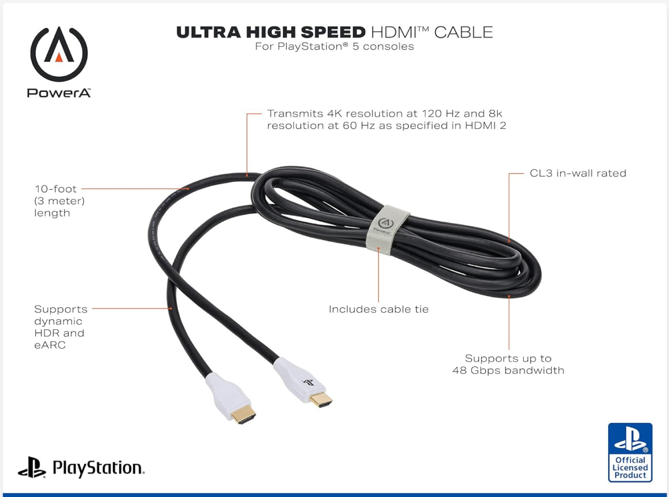
Figure 2: Key features and specifications of the HDMI cable.
