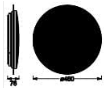
Image: Technical drawing showing the dimensions of the LEDVANCE ORBIS SPARKLE SMART+ WiFi Ceiling Light (Ø 460mm, height 76mm).
