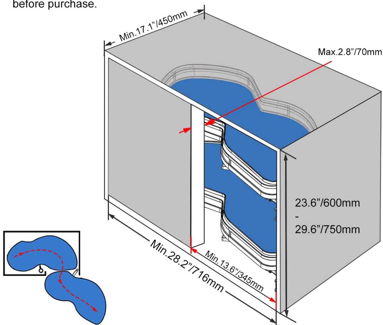
Figure 3: Cabinet space requirements for installation.
