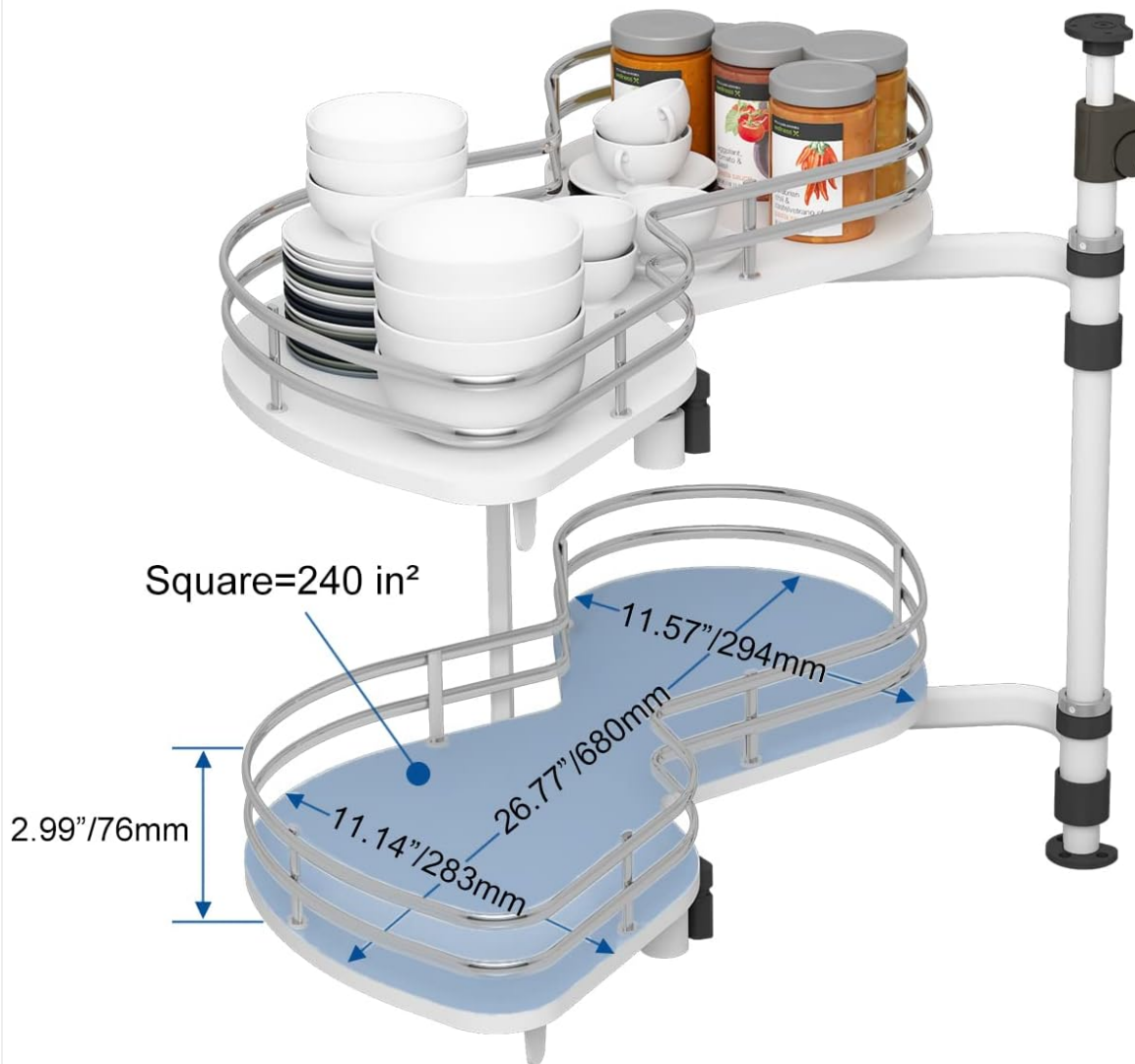
Figure 5: Large storage capacity and dimensions of the trays.
