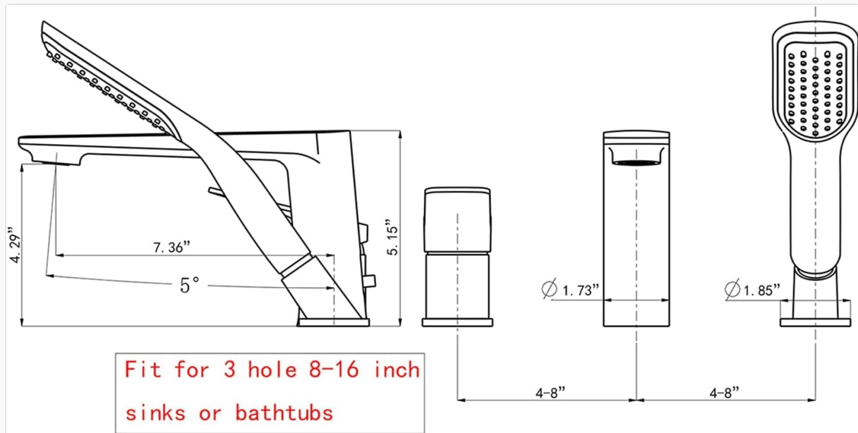
Figure 5.1: Dimensional drawing for installation planning.
