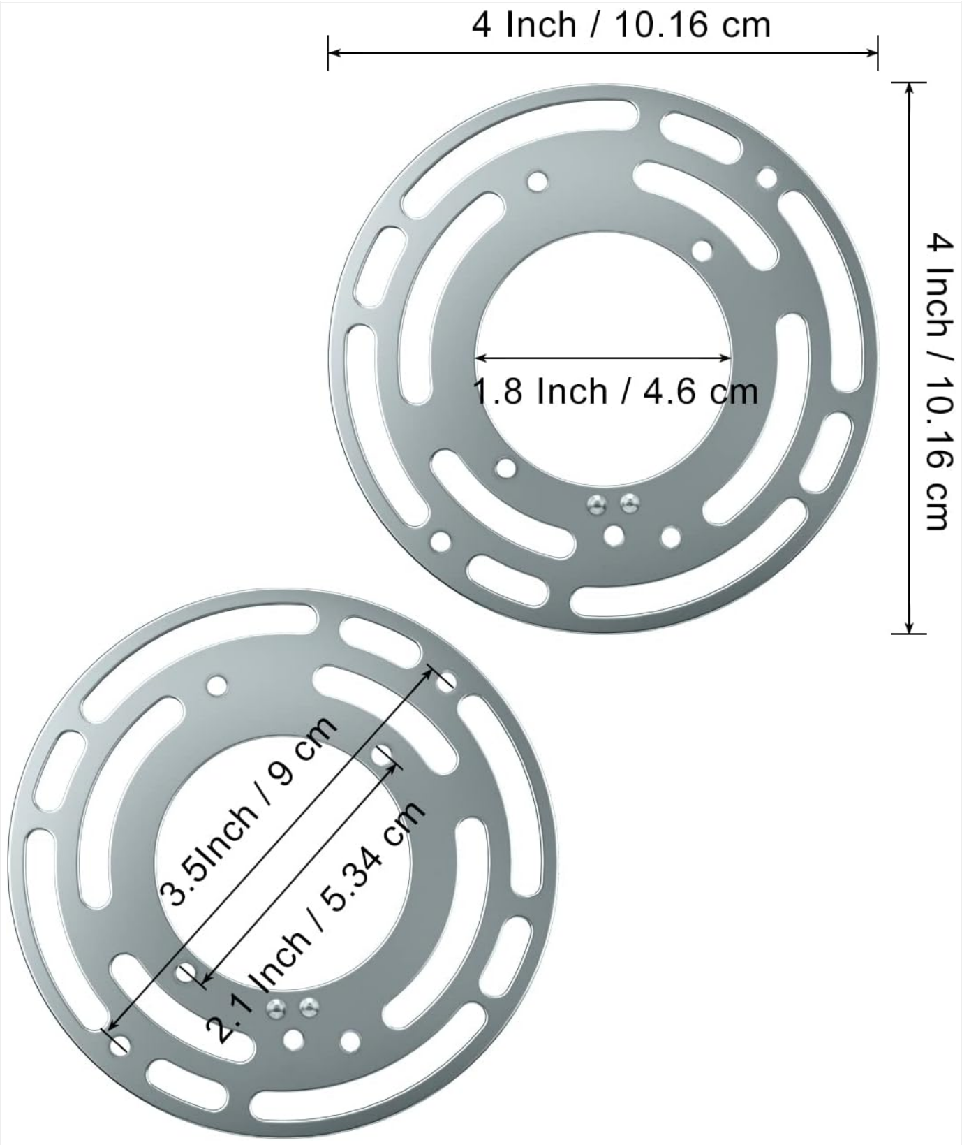
Figure 3: Dimensional specifications of the mounting bracket.
