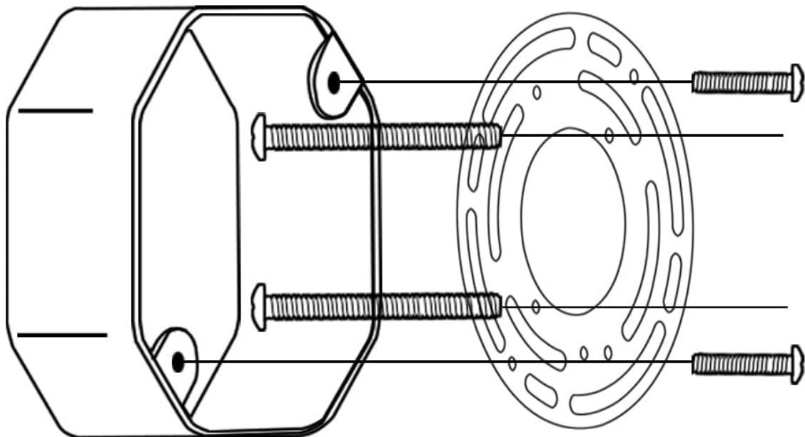
Figure 4: Installation diagram of the mounting bracket to a junction box.
