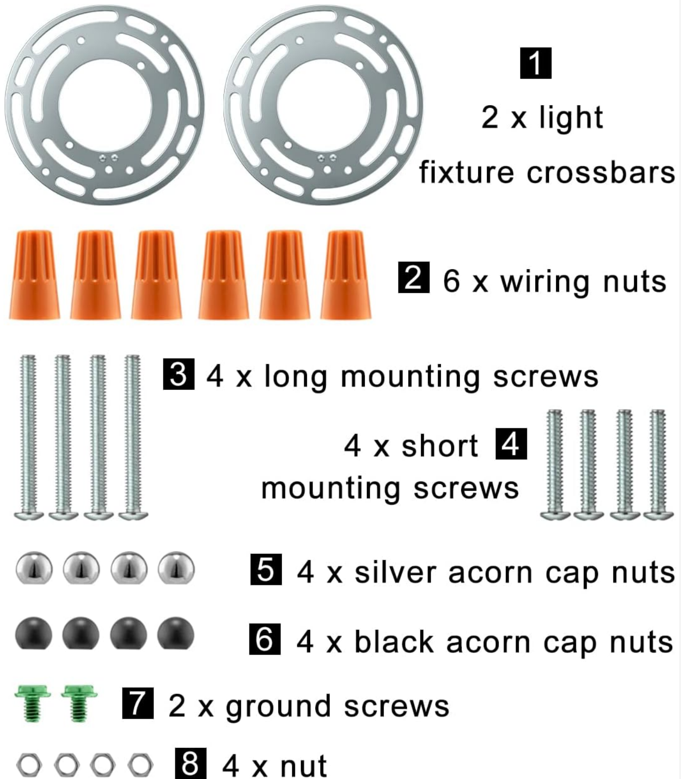
Figure 1: All components included in the package, clearly labeled.
