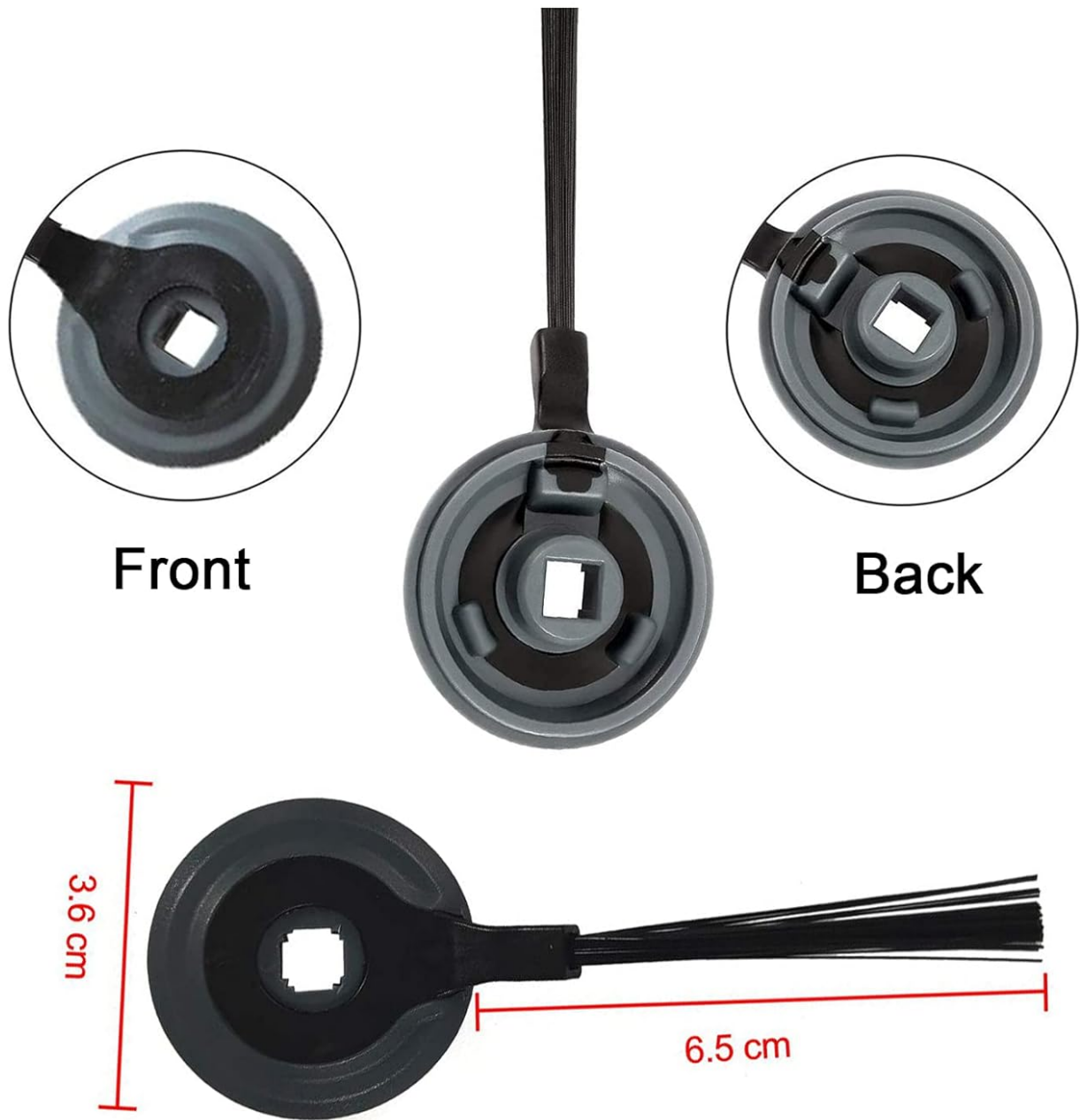
Figure 2: Detailed views of a single side brush, illustrating its front, back, and approximate dimensions (3.6 cm base width, 6.5 cm brush length). This image helps in identifying the correct replacement part.
