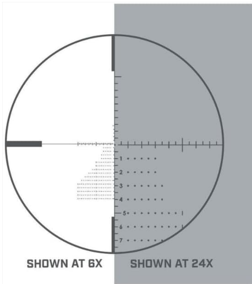
Figure 4: Illustration of the First Focal Plane reticle, showing its appearance at 6x and 24x magnification.
