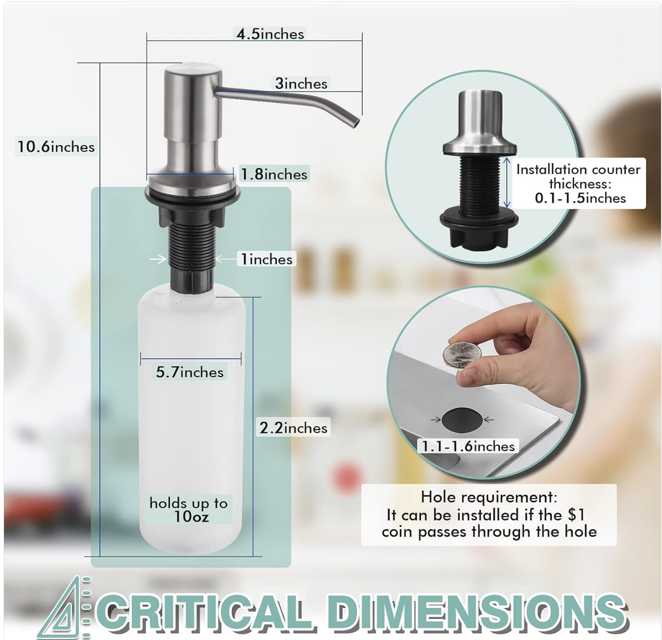
Image 4.2: Critical dimensions for the integrated soap dispenser.
