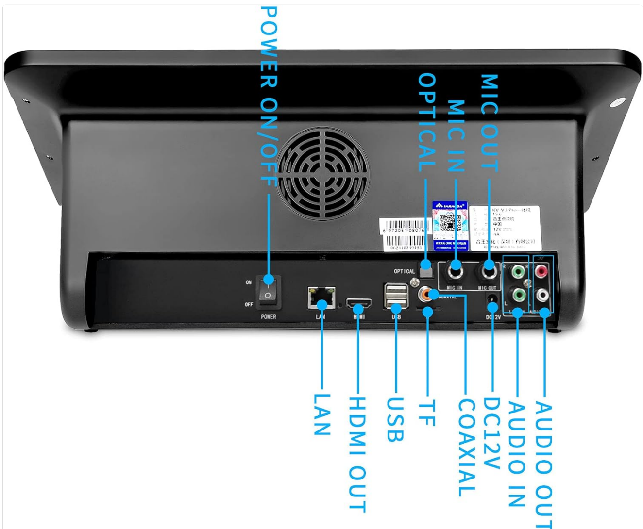
Image description: Rear view of the karaoke system showing various input/output ports including Power, Optical, Mic In, Audio In, Audio Out, DC 12V, Coaxial, TF, USB, HDMI Out, and LAN.
