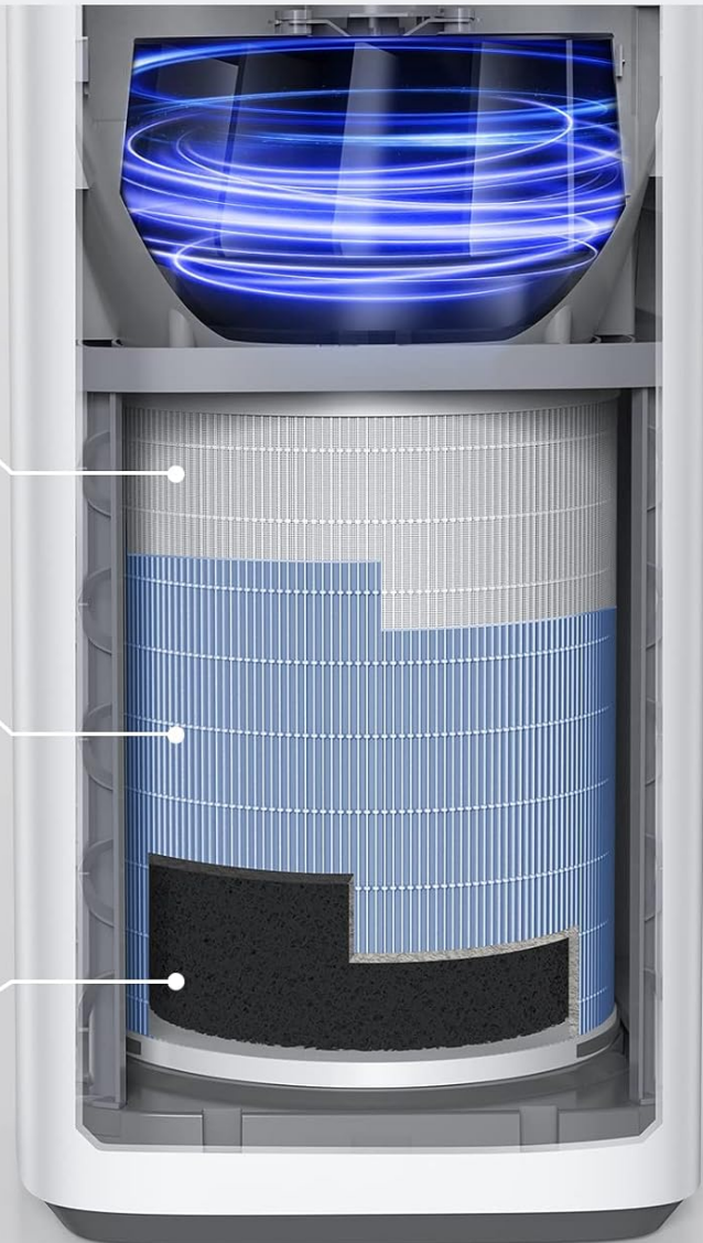
Figure 3: 3-Stage Filtration System components.
