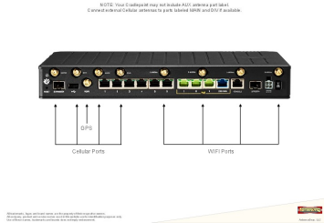
Cradlepoint E3000 Router External Antenna Ports
