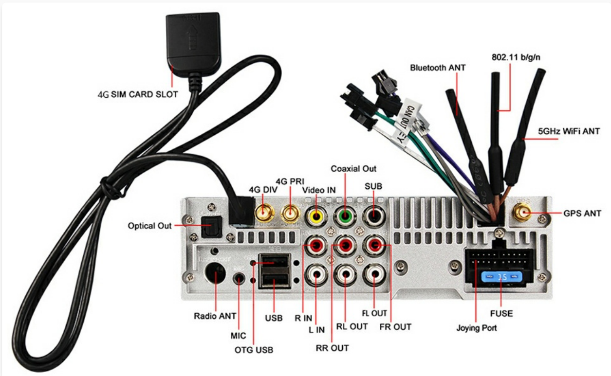
Dimensions and included accessories for the JOYING car stereo.
