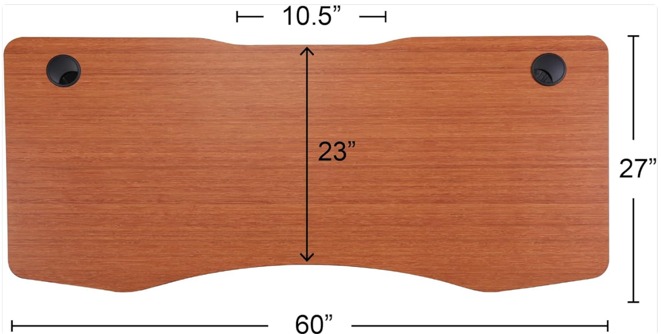
Figure 3: Integrated Cable Management Tray
