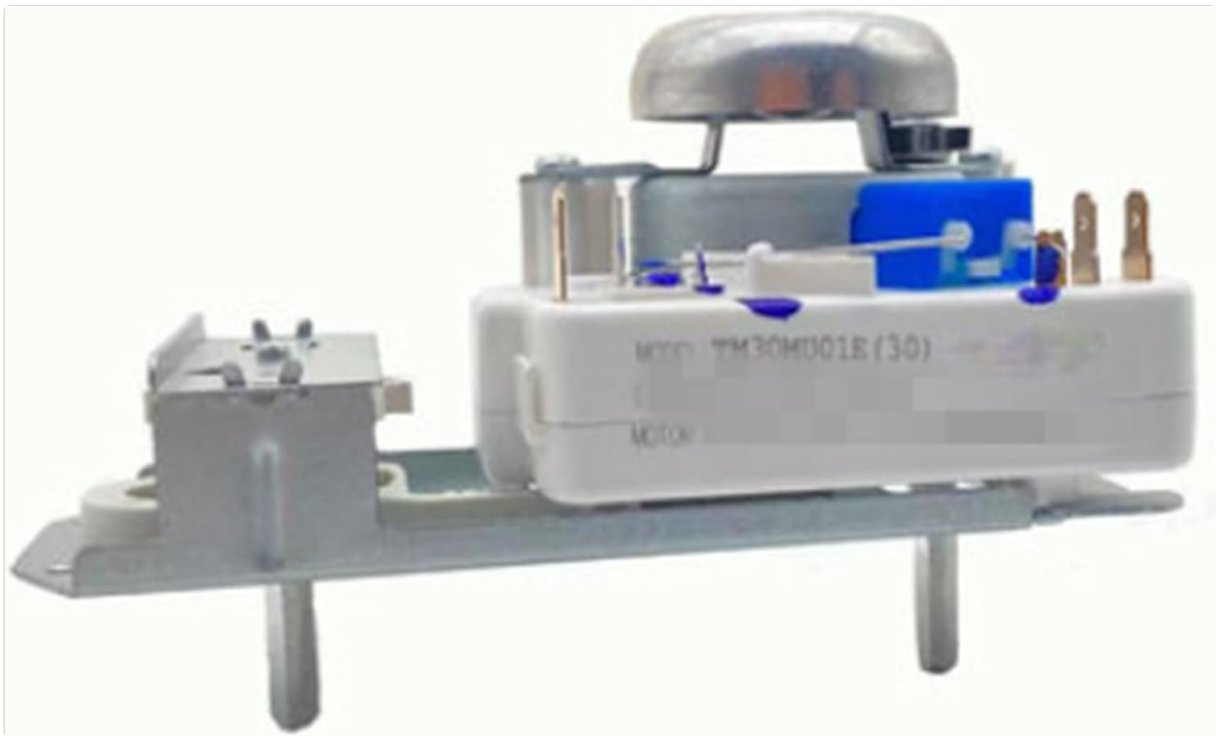
Figure 1: Main view of the zatagen TM30MU01E Microwave Timer, showing its overall structure and electrical terminals.
