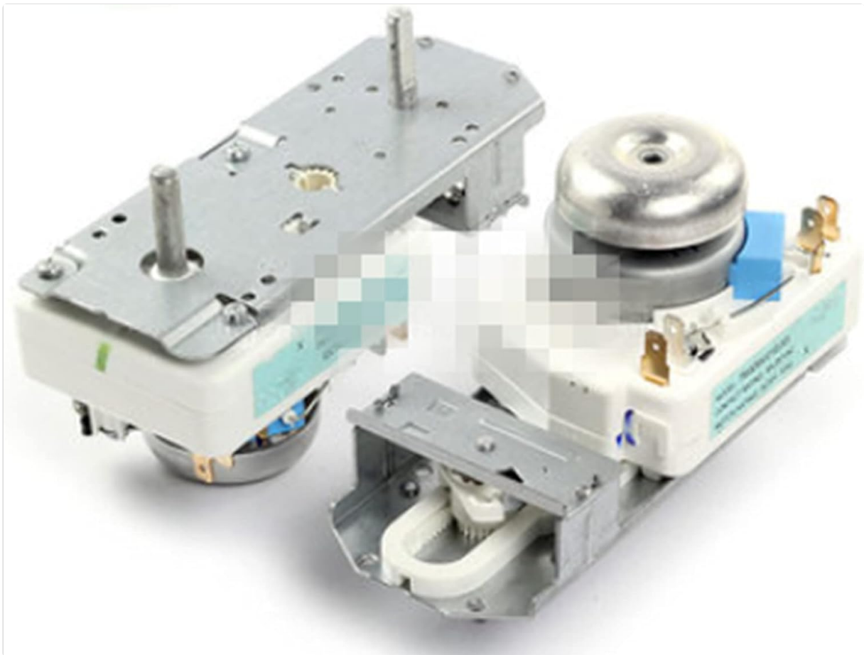
Figure 3: Multiple views of the timer, illustrating its internal mechanism and mounting bracket design.
