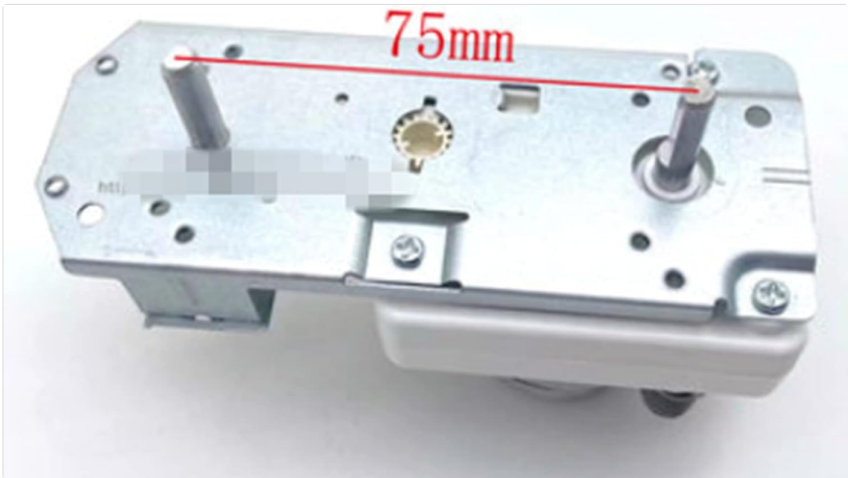
Figure 2: Top-down view of the timer, highlighting key dimensions for compatibility assessment. The distance between mounting posts is approximately 75mm.
