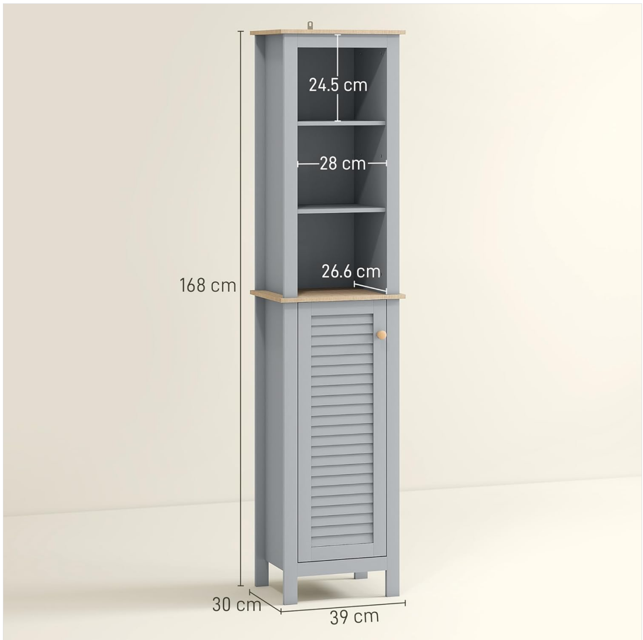
Figure 5: Product Dimensions. This diagram provides detailed measurements of the cabinet, including overall height, width, depth, and individual shelf dimensions.
