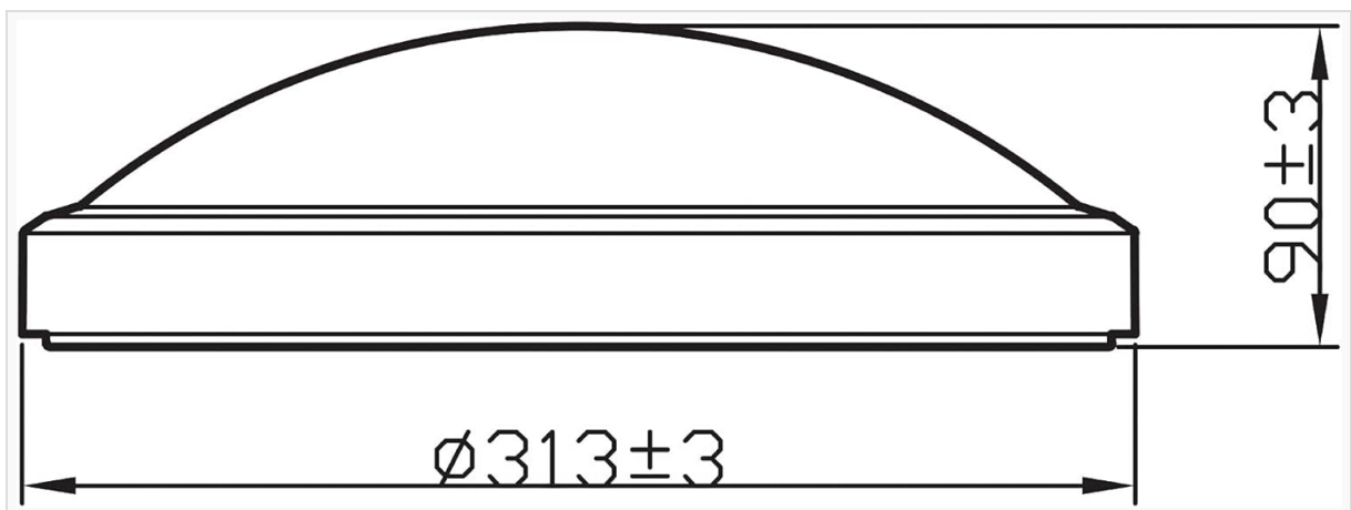
Technical drawing illustrating the dimensions of the Philips DORIS LED Ceiling Light, with a diameter of 313mm and a height of 90mm. Refer to this for precise installation planning.
