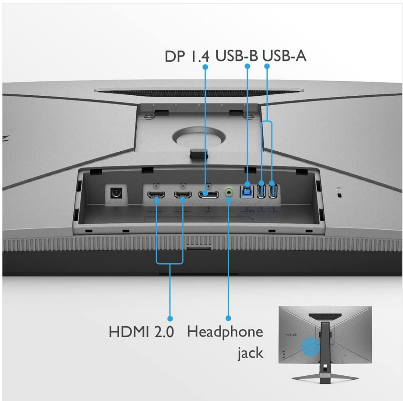
Figure 3.1: Rear panel connections including HDMI, DisplayPort, USB-B, USB-A, and Headphone Jack.
