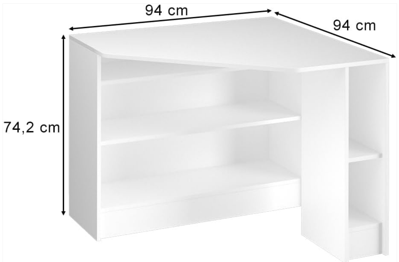
Image 2.2: Detailed dimensional drawing of the Alvaro Corner Desk.
