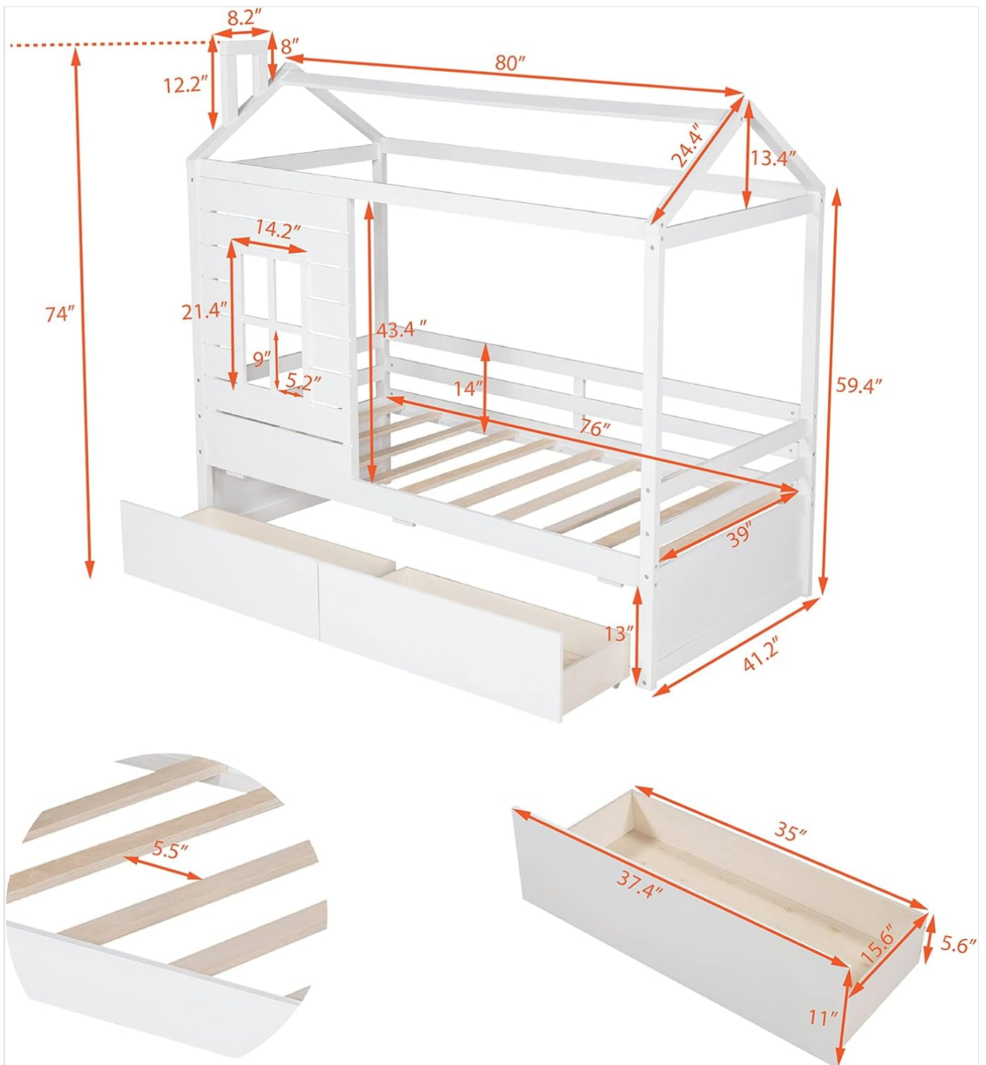
Image: Detailed dimensions of the Twin House Bed, including height, length, width, and internal measurements for the mattress and drawers.
