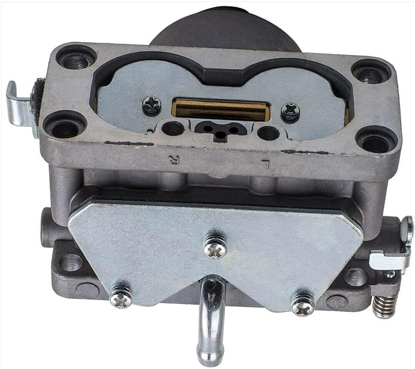
Figure 3: Side view of the carburetor, highlighting the fuel inlet and mounting flange.
