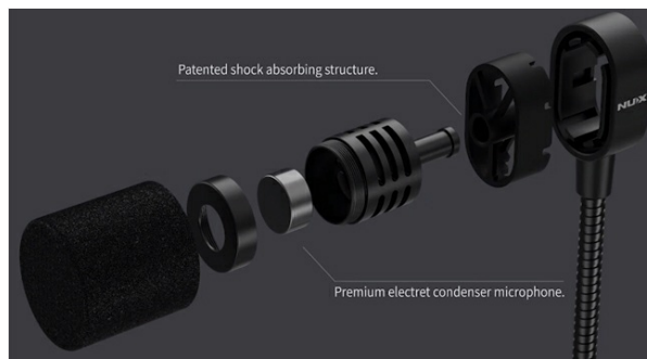
Image: An exploded diagram showing the internal components of the NUX B-6 microphone, including its premium electret condenser and patented shock-absorbing structure.
