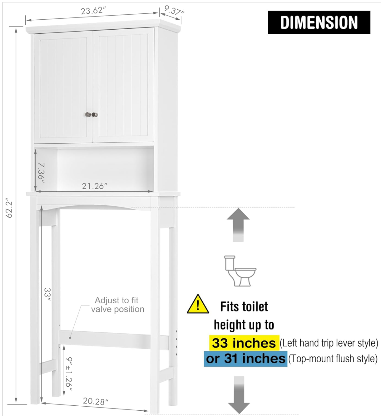
Image 8.1: Product dimensions and toilet clearance.
