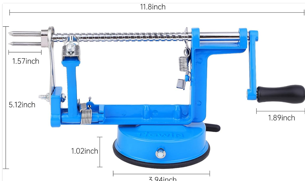
Figure 7.1: Product dimensions.
