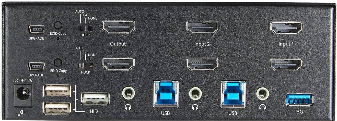
Figure 2: Rear Panel Layout
