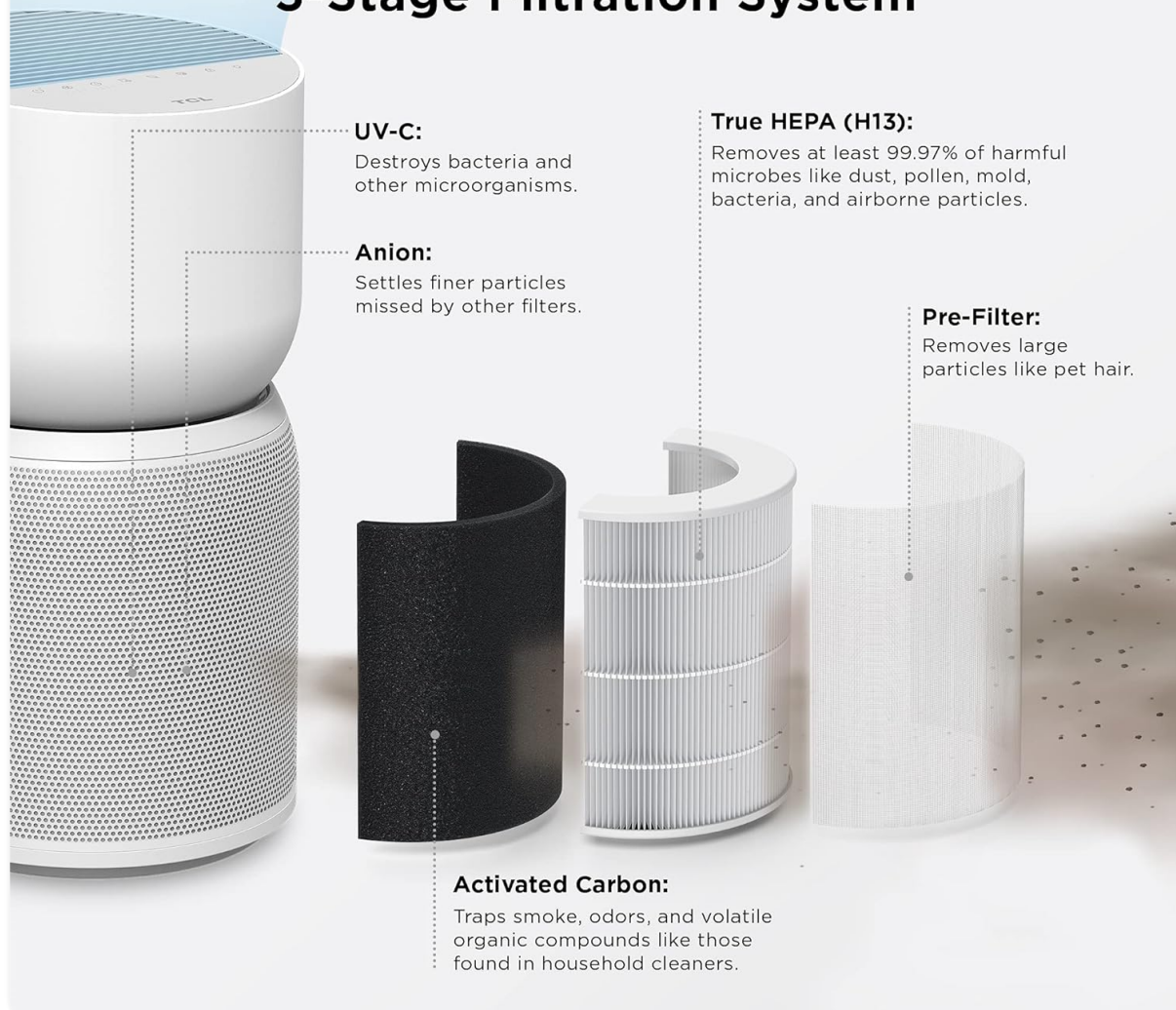
Figure 5: The 5-Stage Filtration System components.
