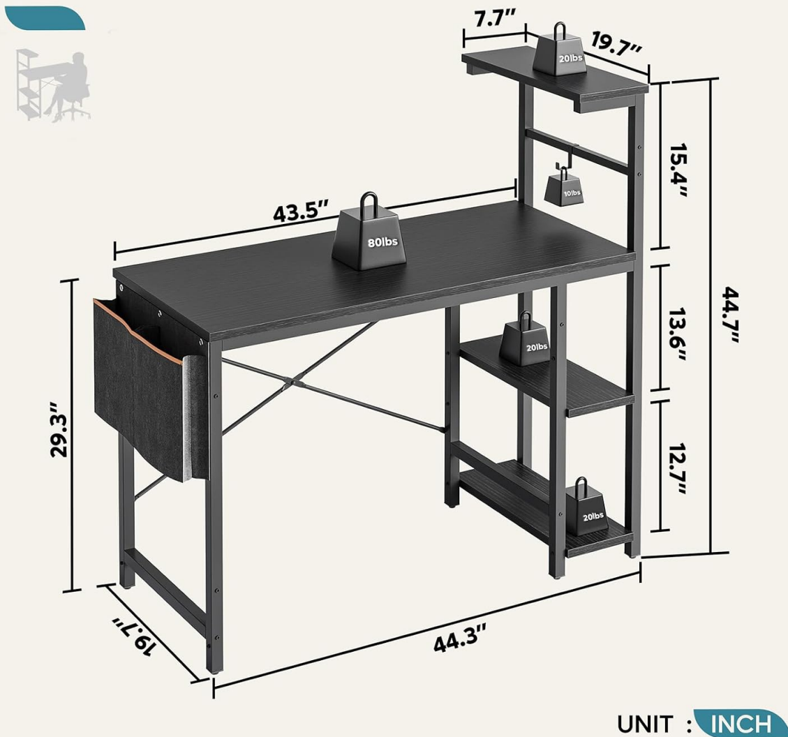
Image 4: A detailed diagram illustrating the product dimensions and weight capacities for various sections of the Bestier Gaming Desk.
