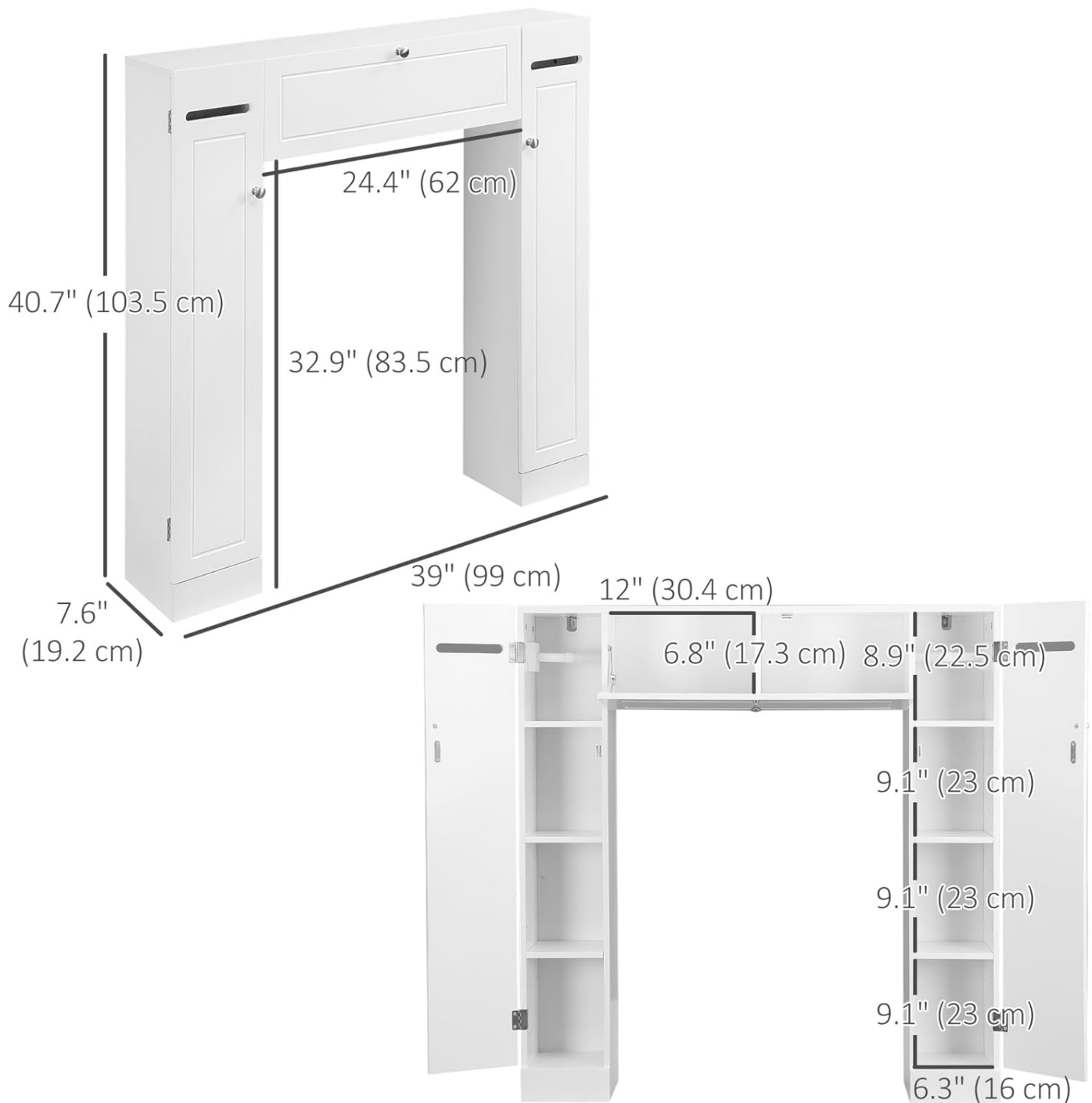
Image: Detailed dimensions of the kleankin over-the-toilet storage cabinet.
