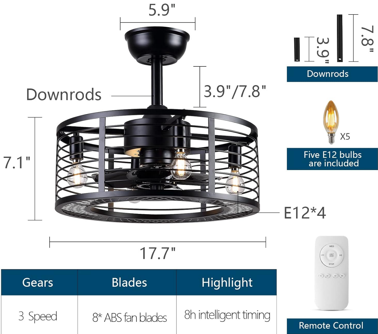
Figure 4.1: Product Dimensions and Components Overview
