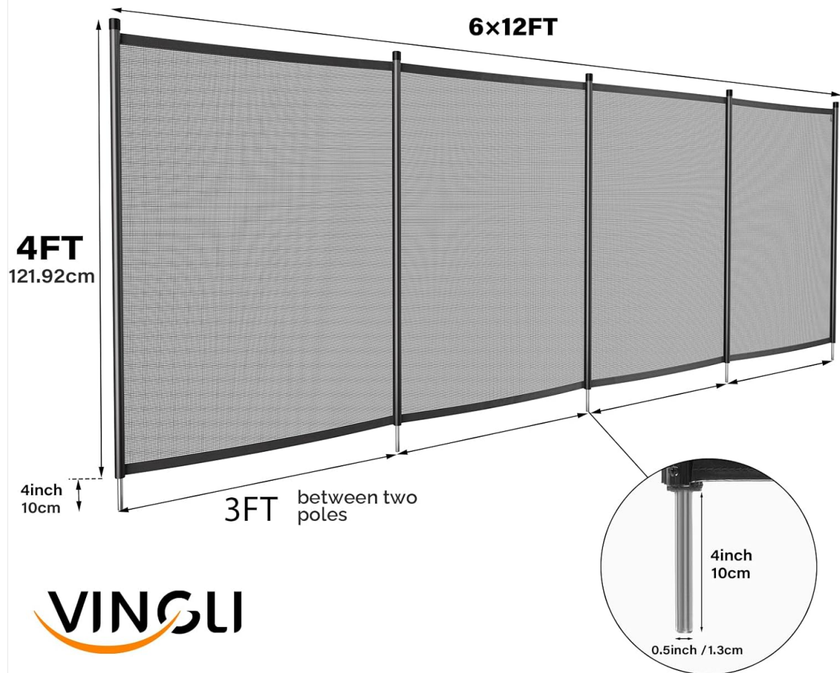
Image: Diagram illustrating the dimensions of the VINGLI pool fence, showing 4 feet height and 12 feet panel length, with 3 feet between poles.
