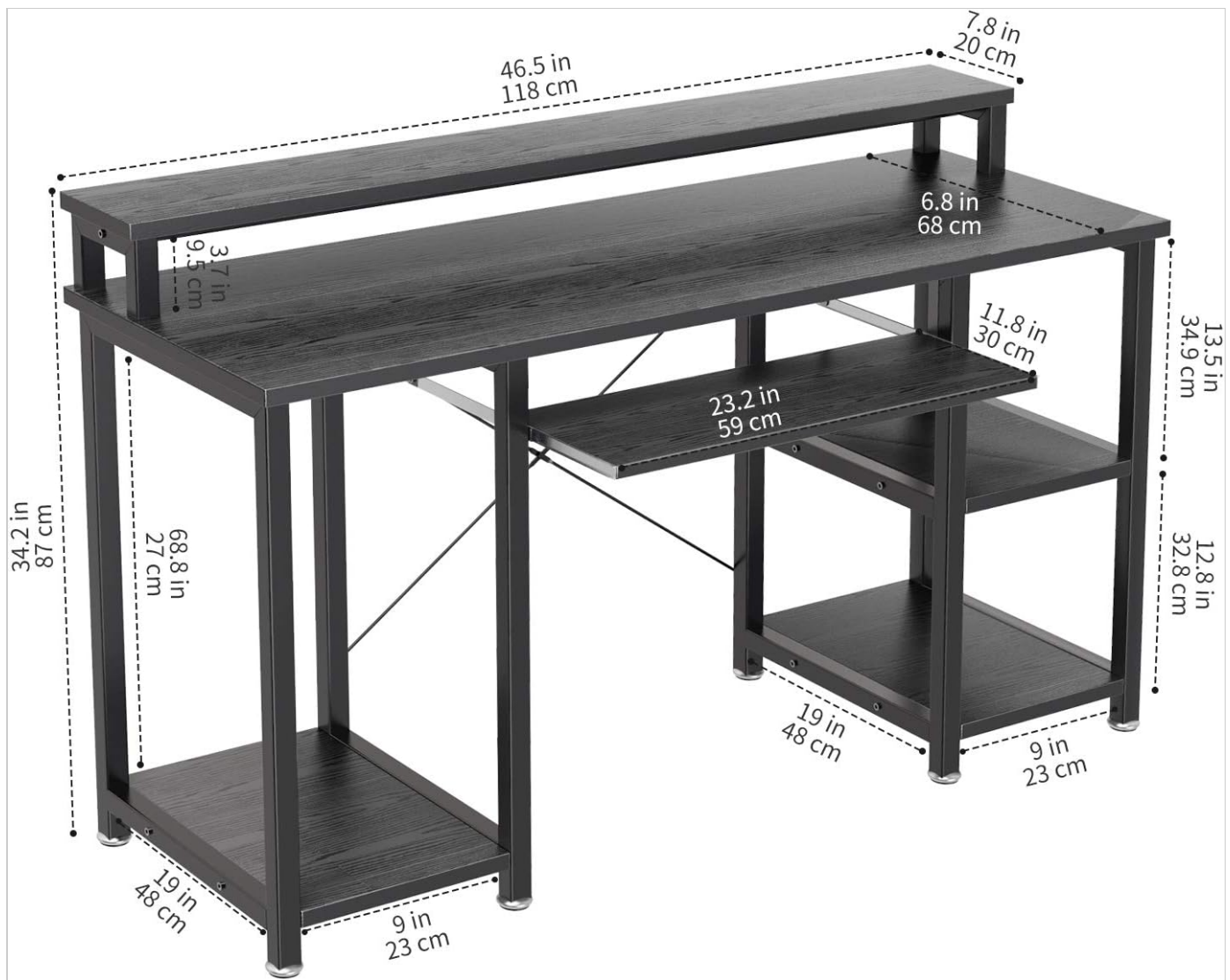
Figure 4.1: Dimensional overview of the Marsail Home Office Desk, illustrating key measurements for planning your space.
