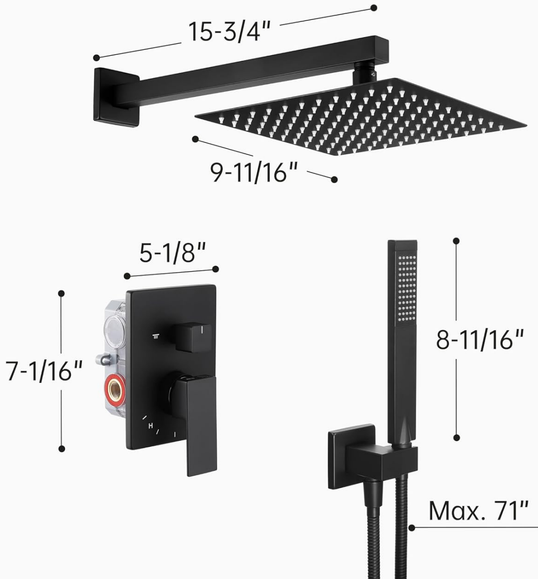
Image: U.S. Standard Connections and dimensions for the shower system components.
