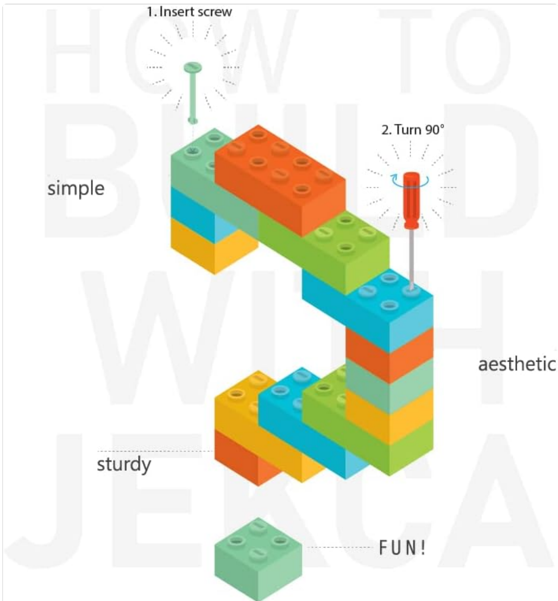
Figure 3.1: Basic interlocking mechanism. Insert the pin (screw) into the block and turn 90 degrees with the pin driver to secure it.
