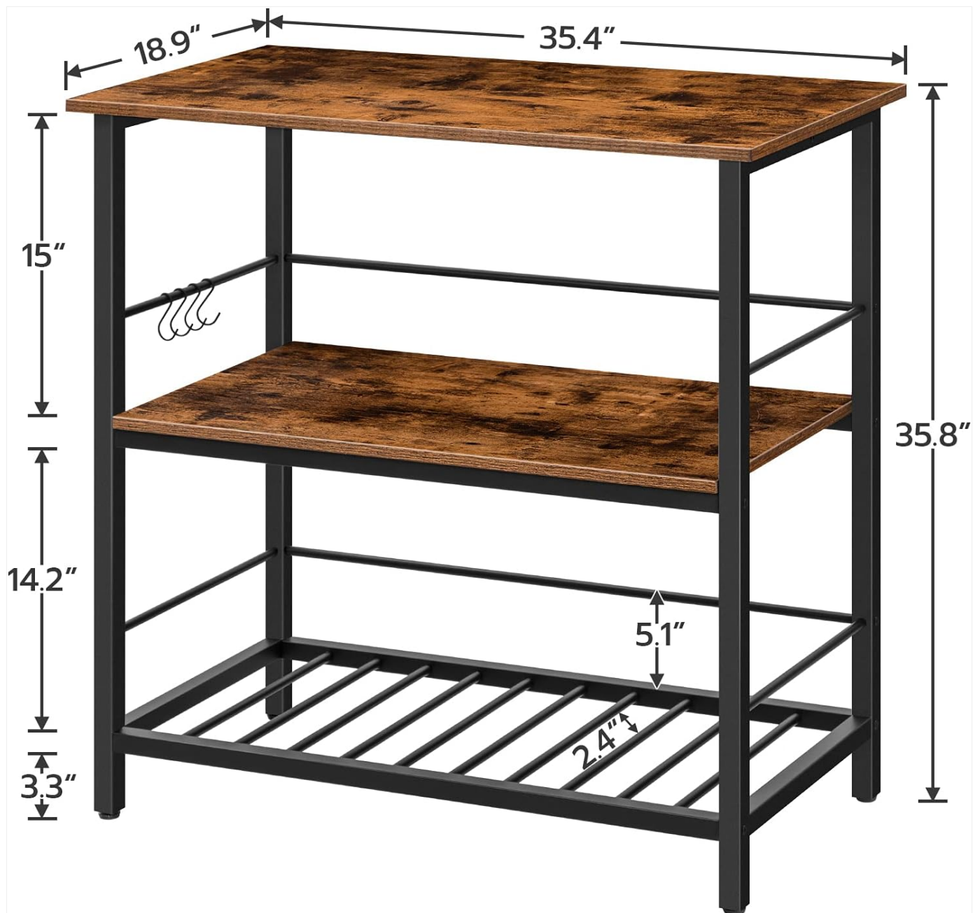
Image: Detailed dimensions of the HOOBRO Kitchen Island, showing its height, width, and depth, as well as shelf spacing.
