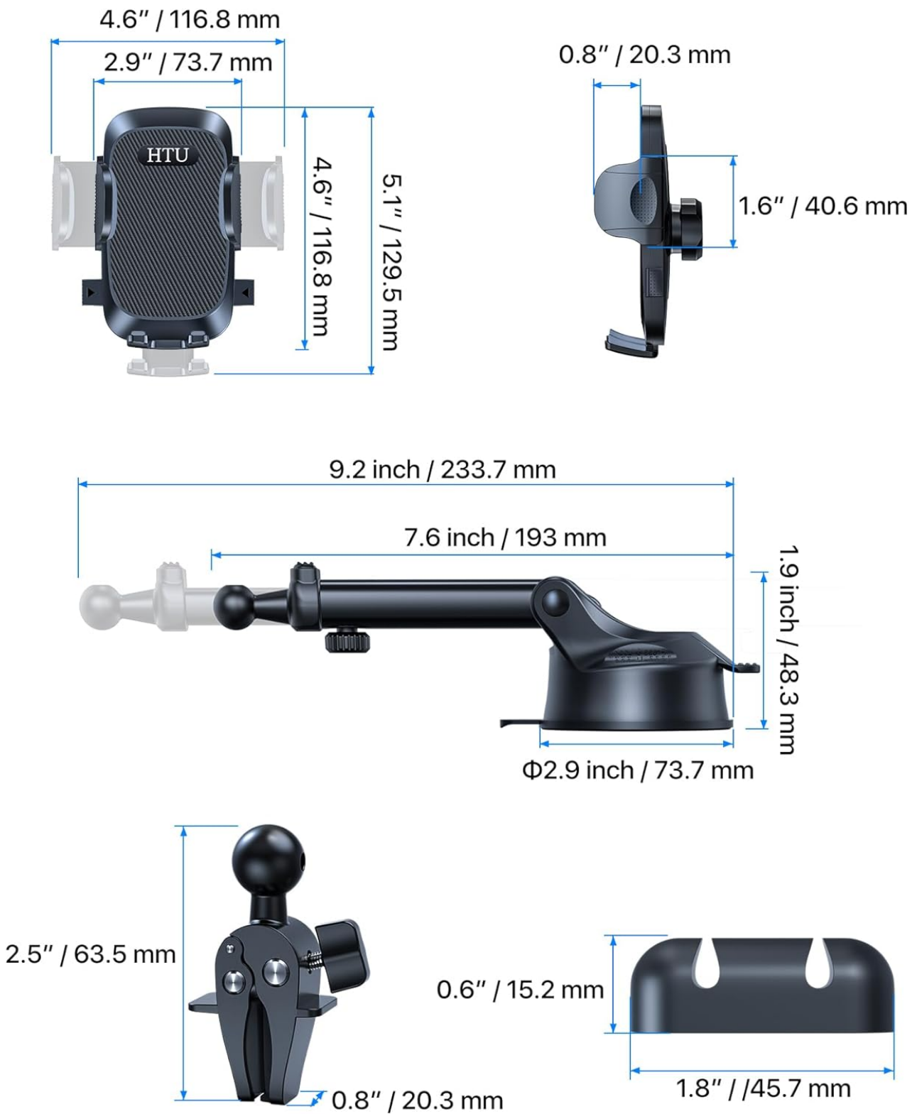
Figure 7.1: Product Dimensions
