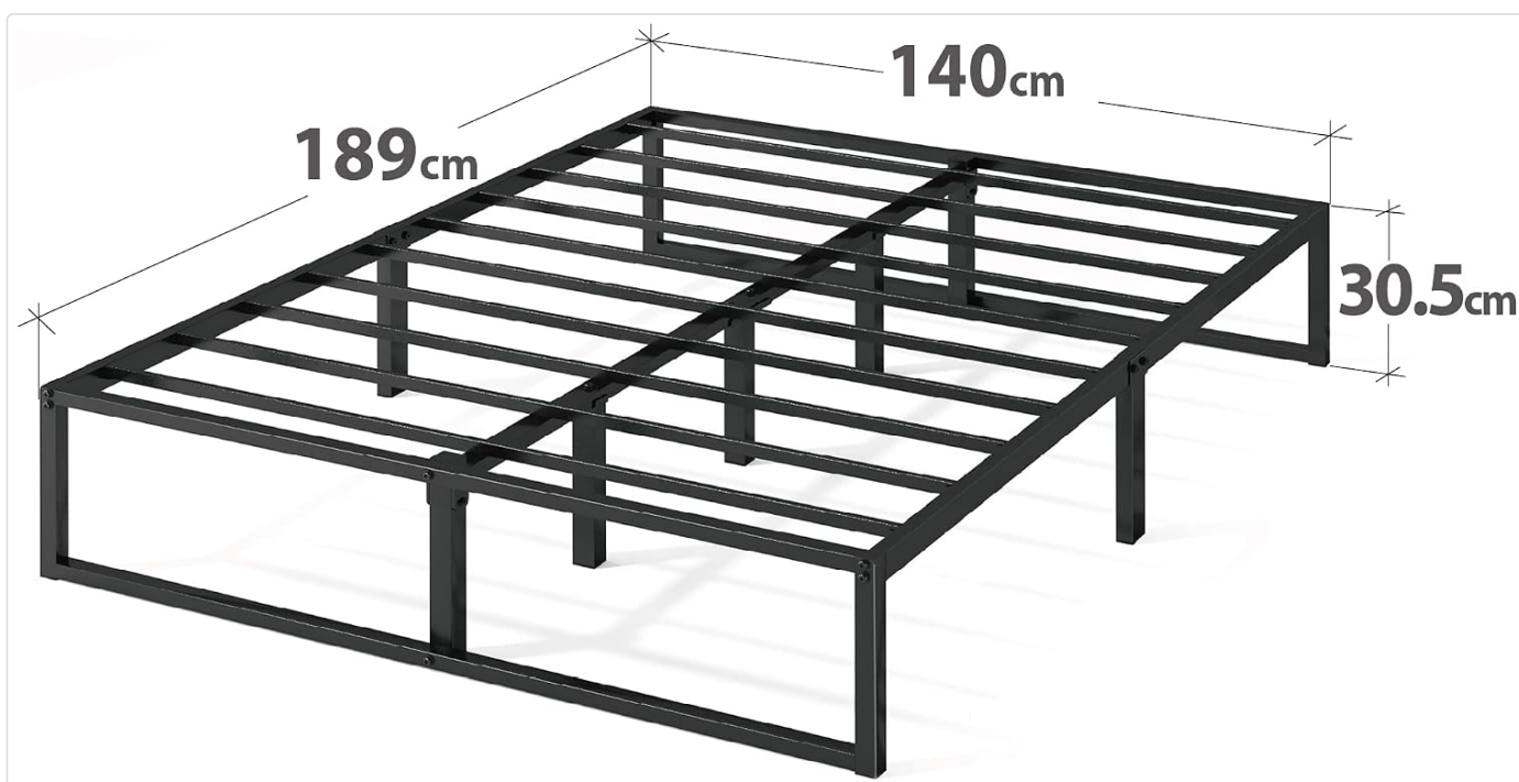
Figure 6: Detailed dimensions of the Zinus Lorelai bed frame.
