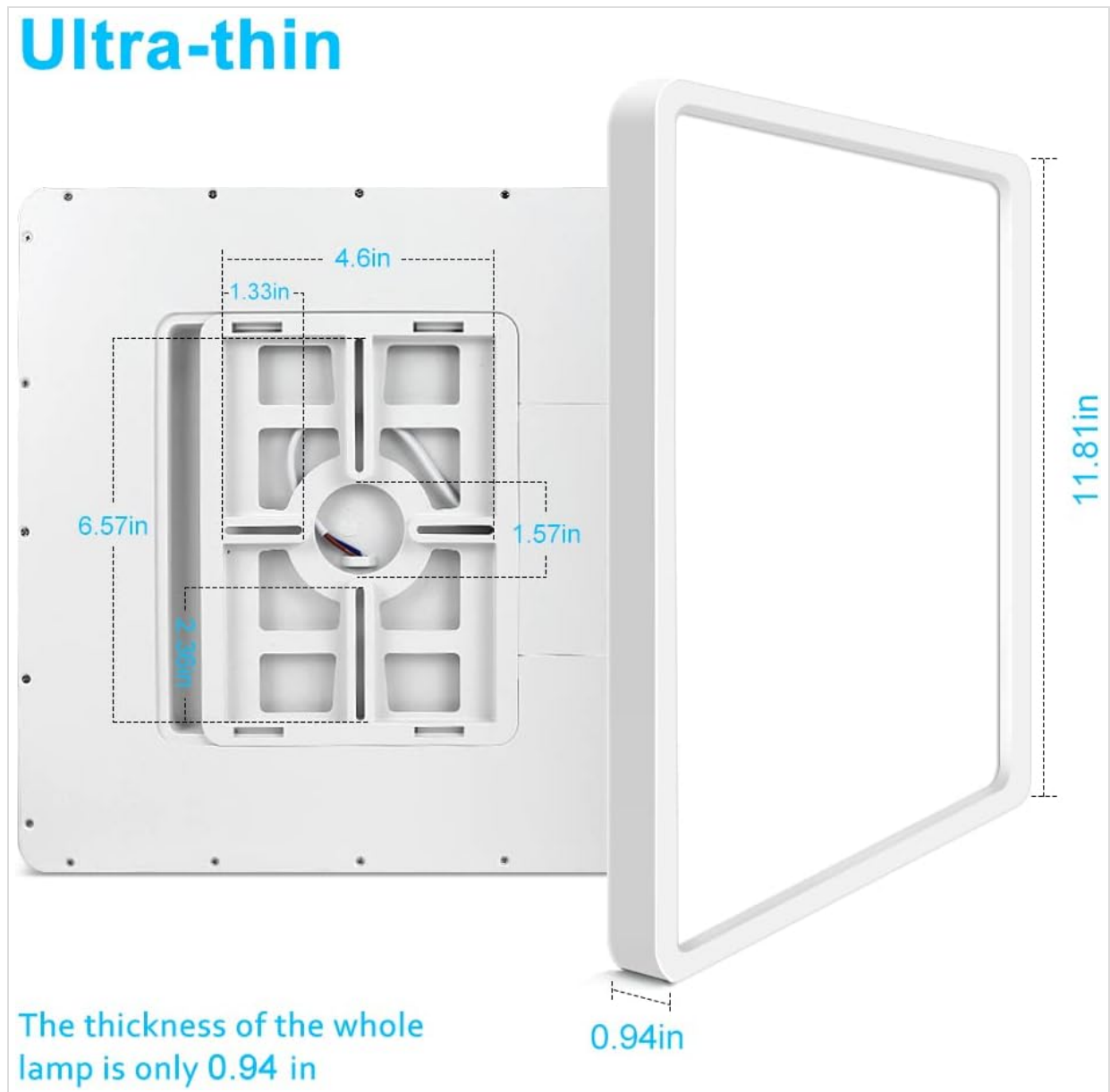
Image 4: Detailed dimensions of the light fixture, highlighting its 0.94-inch thickness.
