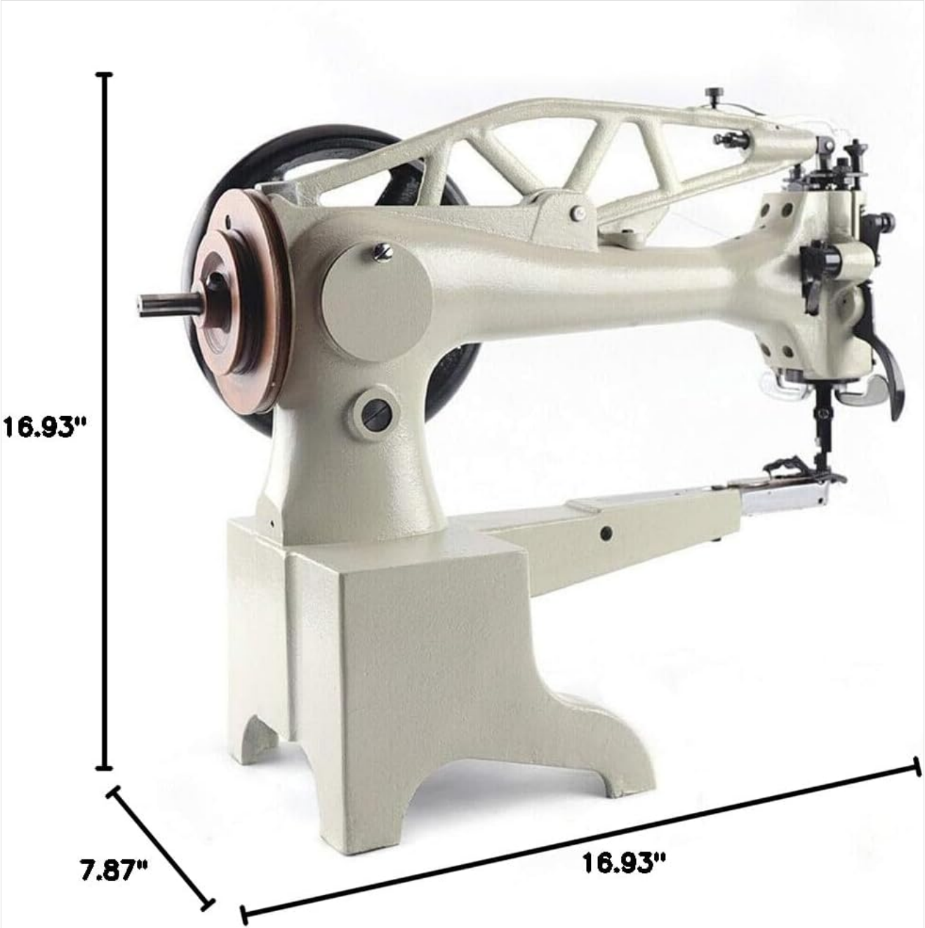
Image: A diagram illustrating the key dimensions of the YIYIBYUS SM-2972 Hand Crank Industrial Patcher Sewing Machine.
