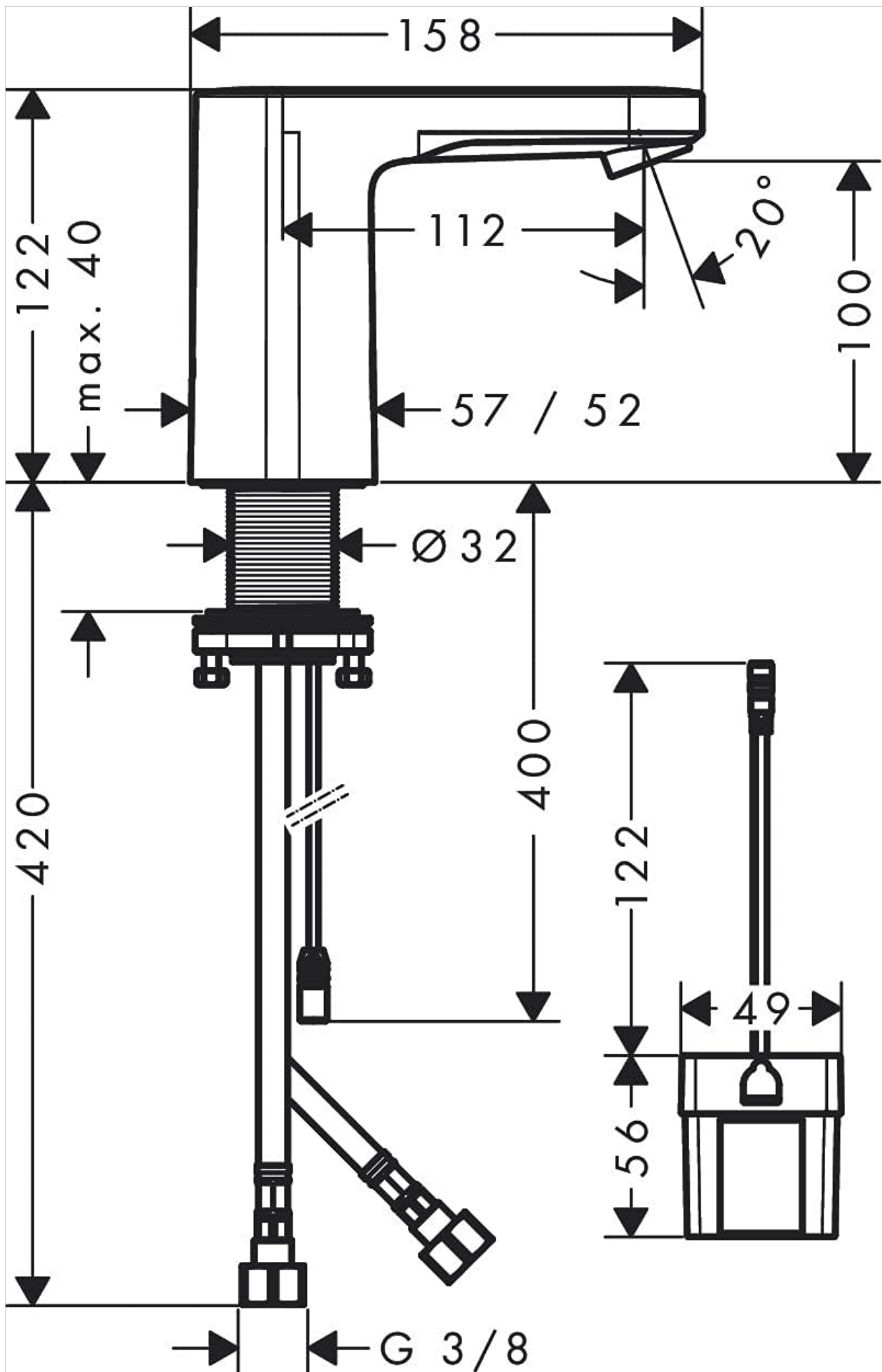
Image: Technical drawing with dimensions (in mm) for installation planning.
