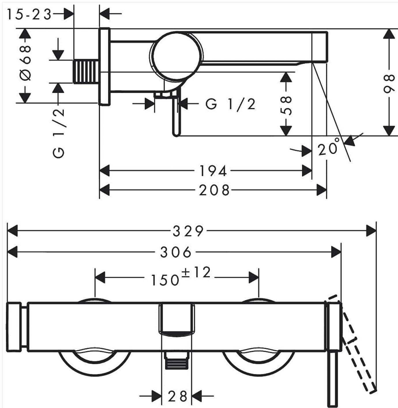
Image 2.1: Technical drawing showing dimensions and connection points for installation.
