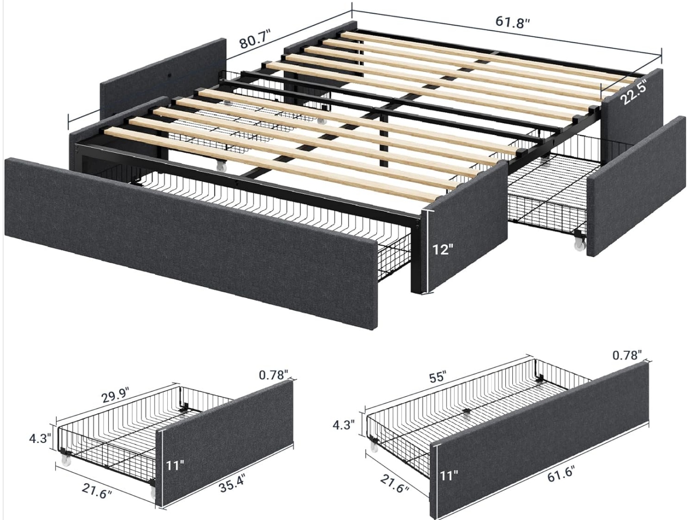
Image 3.1: Exploded view of the bed frame components, illustrating the main parts including the frame, slats, and storage drawers.
