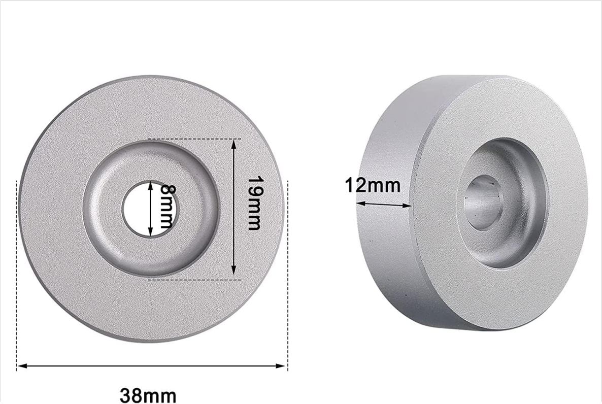
Image 6.1: Diagram illustrating the dimensions of the 45 RPM adapter.
