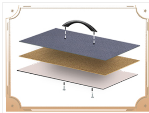
Figure 2: Exploded view of a fabric drawer, illustrating the non-woven fabric and MDF board construction for durability.
